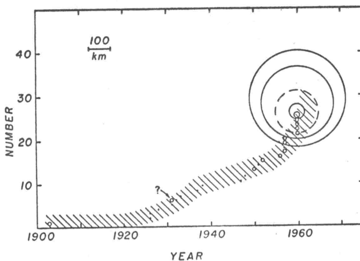
FIGURE 1.—Trend of the acceptance of structures as being of meteoritic origin. Aerial photography after World War II contributed several new finds. Small dots refer to craters less than 1 km diameter, open dots to those between 1 and 30 km, and the large circles are to the scale shown. A few are multiple, but are not so plotted.
